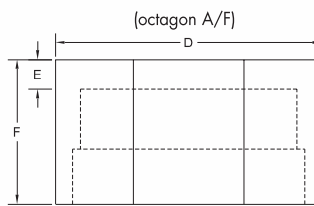
Insulating cap
